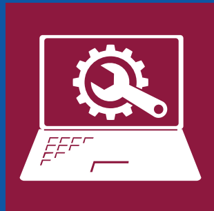
Software Tools
