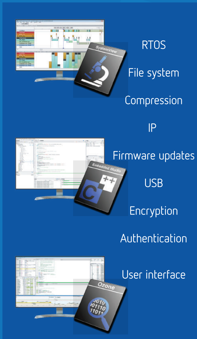
Software Tools
